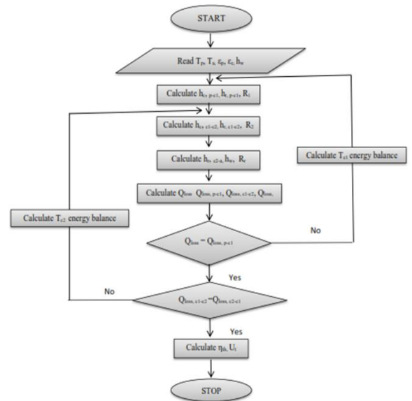
Figure 1. Flow Chart
