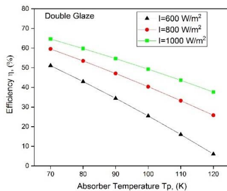
Fig. 5: Efficiency v/s Absorber temperature at different insolation
