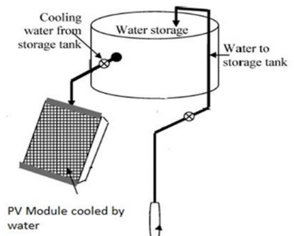
Fig 3. Experimental set-up, A schematic [29]
